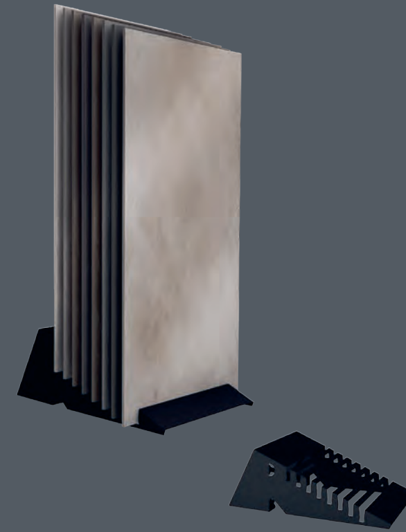
BASIC FOLDABLE DISPLAY | CULLA 8 Size: 80x85x2cm Weight: 3,75 kg Suitable for 8 pcs in 80x80 cm and /or in 60x120 cm
